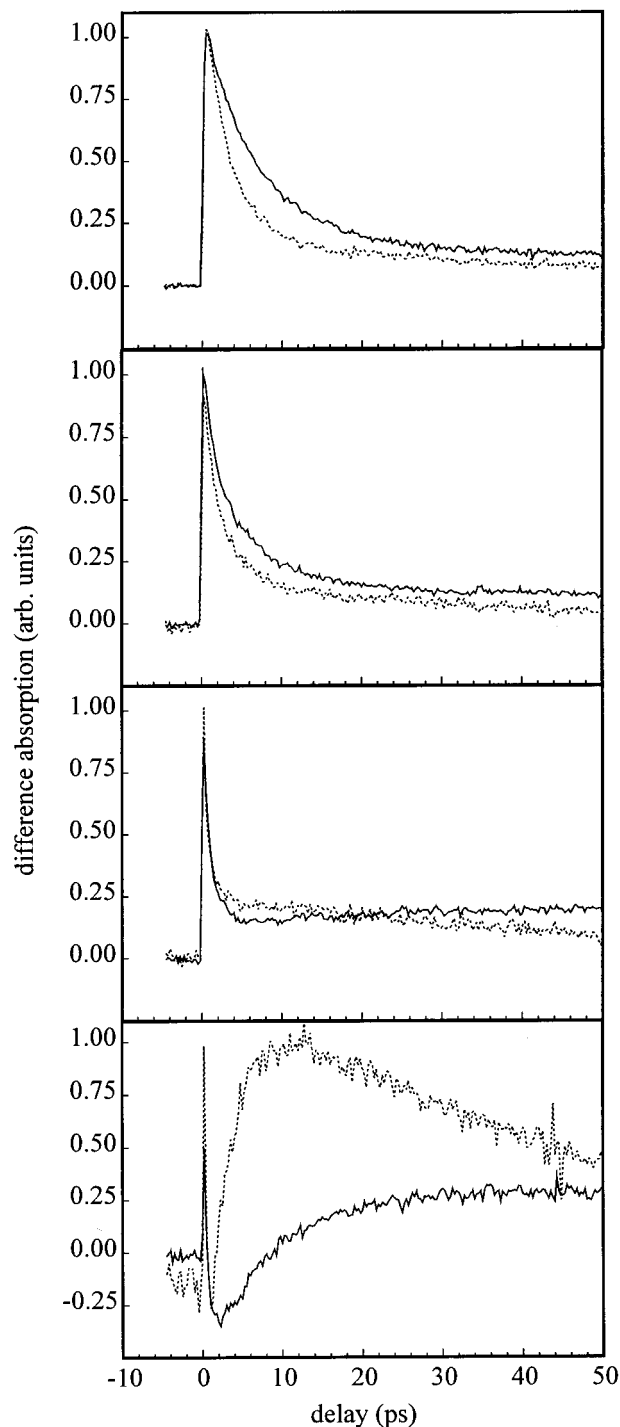
Figure 4. Comparison between the picosecond pump–probe transients of TPE in cyclohexane (solid line) and ethanol (dashed line). The probe wavelengths are 500, 550, 600, and 650 nm (from bottom to top). For all alcohols, the decay in the red part of the spectrum is related to the rise of the signal in the green. For cyclohexane, no such relation is found.
