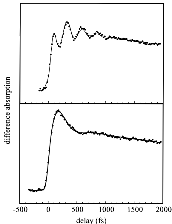
Figure 3. Fits (solid lines) to the two type of oscillations observed in the short-time pump-probe spectra of TPE (dots). In the upper panel the result is shown for the 650 nm transient of TPE in cyclohexane and in the lower panel that for the 600 nm transient of TPE in octanol. The parameters of the fits at 650 nm can be found in Table 1 for the different solvents. The parameters for the fits of the much weaker oscillation at 600 nm were, within the experimental error margins, identical for all solvents.
