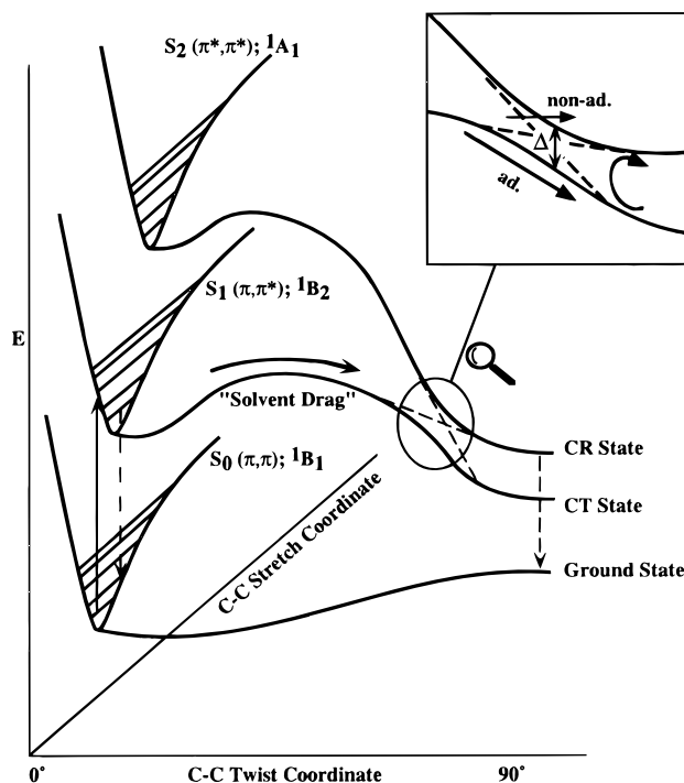
Figure 9. Impression of the excited-state dynamics of TPE. Subpicosecond relaxation occurs along the C–C stretch coordinate, leading to a large Stokes shift between the excitation wavelength (310 nm, solid arrow) and the probed stimulated emission (500 nm, dashed arrow). The subsequent twist around the central bond is strongly hindered by the surrounding solvent. This is indicated as “solvent drag”. The twist leads to adiabatic electron transfer to a zwitterionic state, through an avoided crossing between two excited-state potential surfaces. This is designated by ad(iabatic) in the enlarged crossing region of the inset. The resultant charge-transfer (CT) state is stabilized by solvent reorganization. A very small fraction may cross directly to the upper potential curve (nonad(iabatic) in the inset), which leads to the symmetric charge-resonance (CR) state. In apolar solvents thermal activation of this nonpolar state is possible, and a dynamic equilibrium between the CT and CR states is established.
