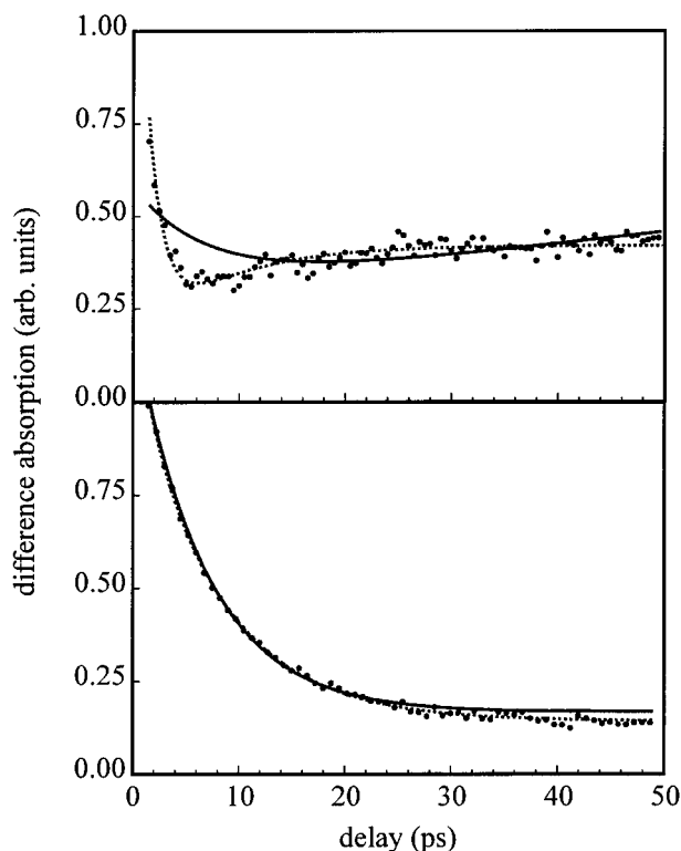
Figure 7. Fits of the 650 nm (upper panel) and 550 nm (bottom panel) transients of TPE in cyclohexane. The fits to the data (dots) of the two-state model (solid lines) are clearly not as good as those of the three-state model (dashed lines). In nonpolar solvents, the transients at all wavelengths can only be simulated consistently, with the same dynamic parameters, when (at least) three states are involved in the dynamics. The parameters of the fits are given in Table 2.
