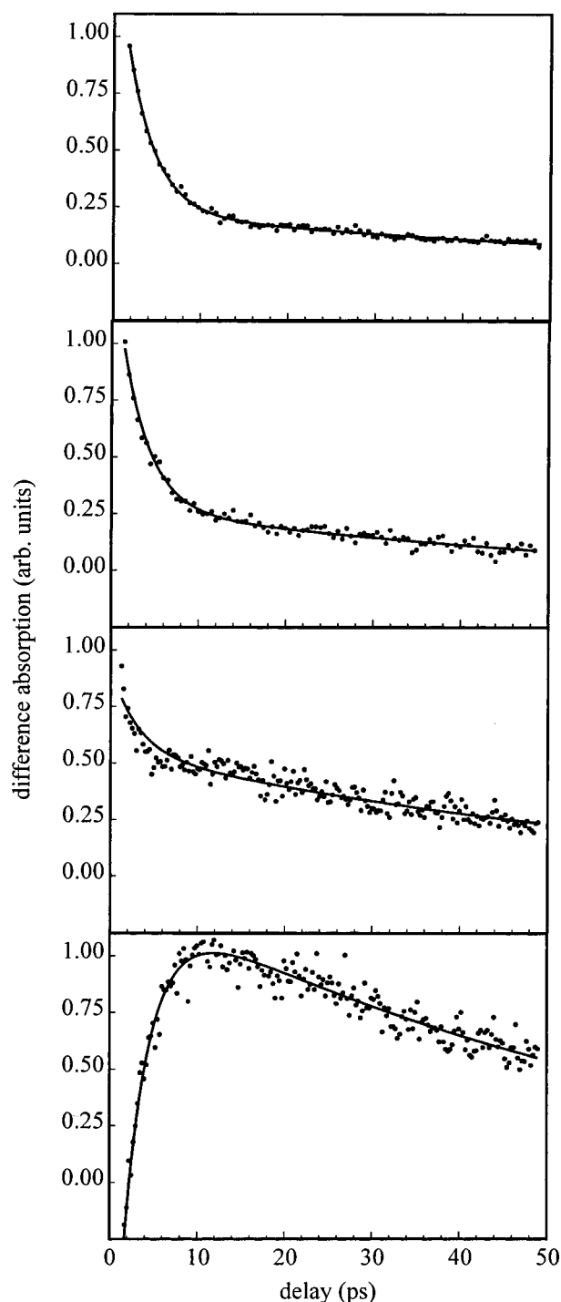
Figure 6. Fits (solid lines) of the 500, 550, 600, and 650 nm transients (from bottom to top) of TPE in ethanol (dots). For simplicity, the solvent independent ultrafast part of the response ( < 2 ps) was excluded from the fitting. A two-state model suffices to explain the data at all wavelengths with the same set of dynamic parameters. These are given in Table 2.
