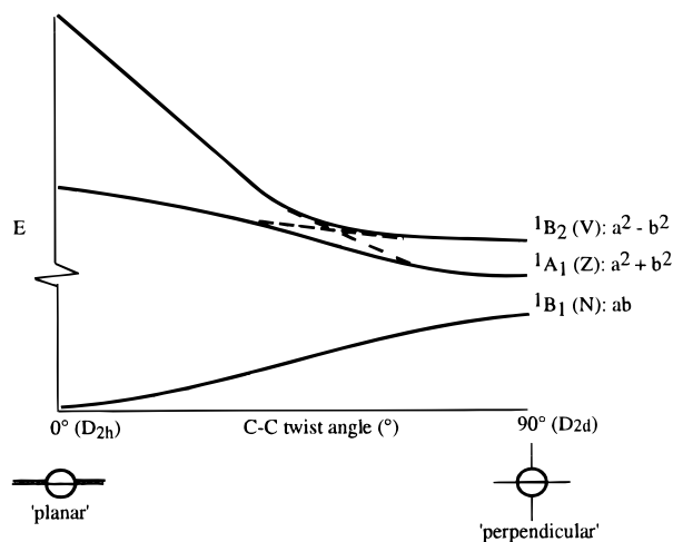
Figure 1. Schematic representation of the lowest potential energy surfaces of symmetric alkenes as a function of the central bond twist angle. Newman projections of the two limiting cases of D_{2h} and D_{2d} symmetry are shown below. The position of the avoided crossing between the two excited states presumably depends on the substituents of the central alkene backbone. The nomenclature of the states (N, Z, V, and ab, a^2 + b^2 , a^2 - b^2 ) is explained in section 3.
