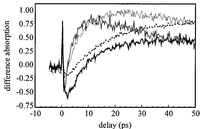
Figure 5. Picosecond dynamics of TPE at 500 nm in ethanol (thin solid line), 1-butanol (dotted line), 1-octanol (dashed line), and cyclohexane (bold solid line). In this part of the spectrum, the pump-probe transients are strongly dependent on the polarity and the viscosity of the liquid, as discussed in the text.
