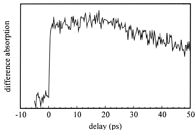
Figure 8. Picosecond dynamics of TPE in ethanol for probing at 450 nm. Apart from a small rise, due to the wing of the 500 nm band, only the overall decay of the excited-state population is observed. Twisting and charge separation do not significantly influence this part of the spectrum.
